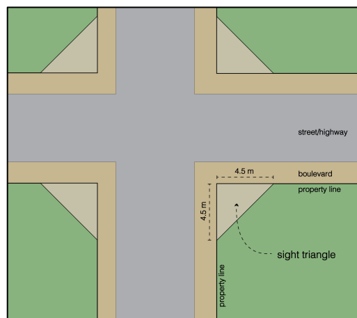
Figure 5. Sight Triangle
