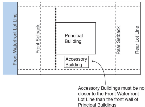
Figure 12. Accessory Building Front Setback Illustration (RM-3 front waterfront)
