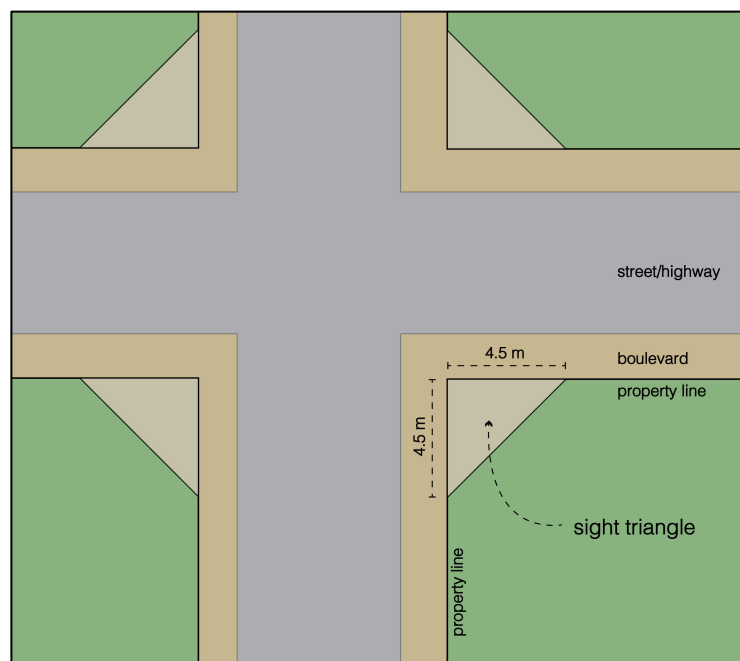
Figure 5. Sight Triangle
