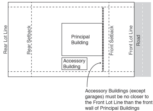
Figure 6. Accessory Building Front Setback Illustration (RS-1 no waterfront)
