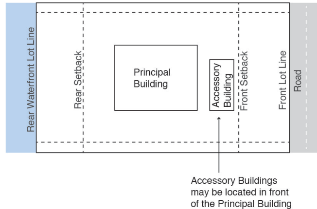
Figure 11. Accessory Building Front Setback Illustration (RM-3 rear waterfront)
