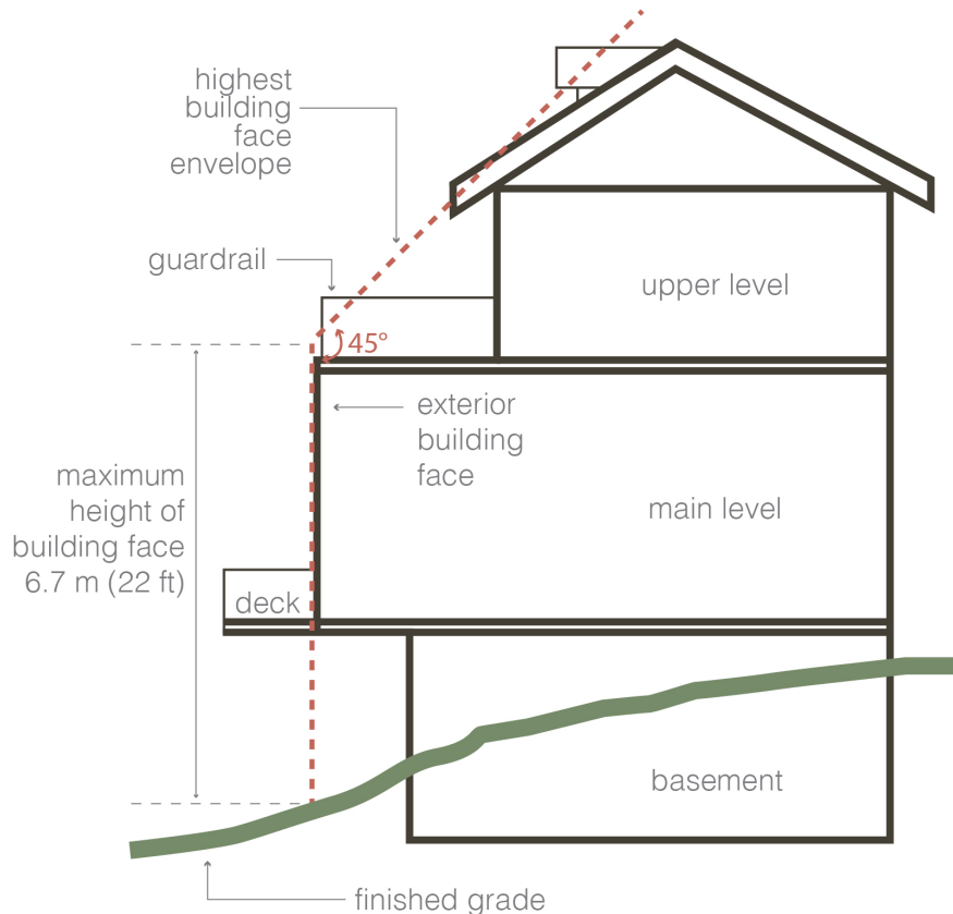
Figure 1. Highest Building Face Envelope
