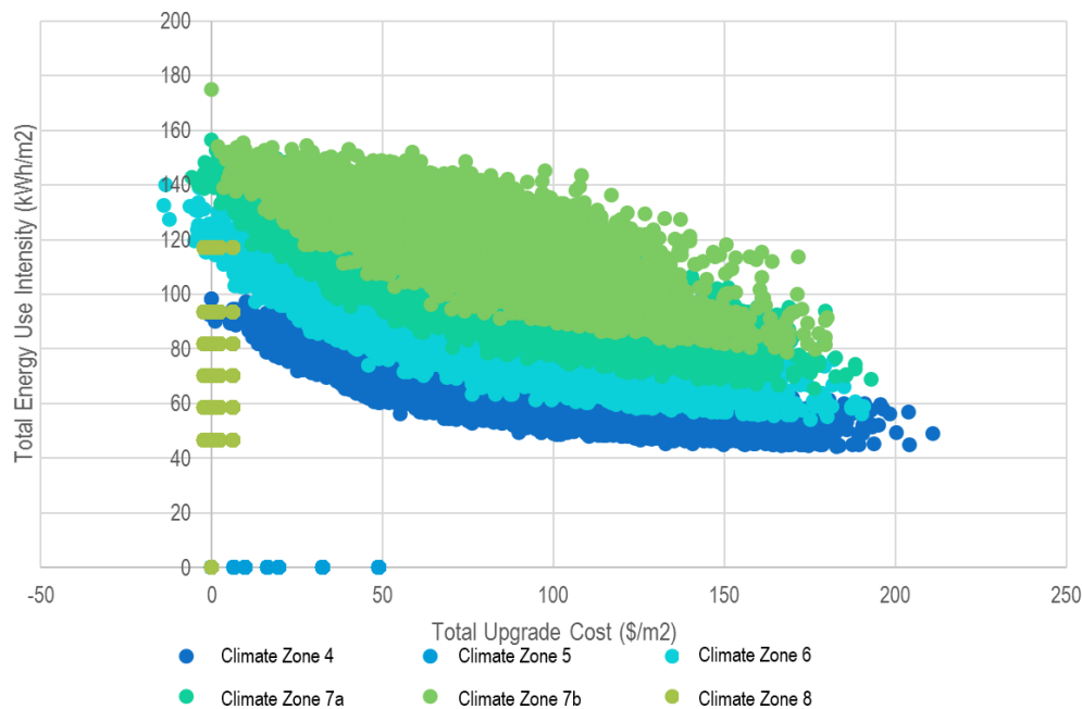
Figure 4: Sample HTAP scatterplot output for the optimization of capital costs for TEDI, Medium SFD
